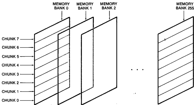
Fig. 5-1. Memory map of T/S 2068.
